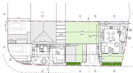
PROPOSED GROUND FLOOR PLAN
