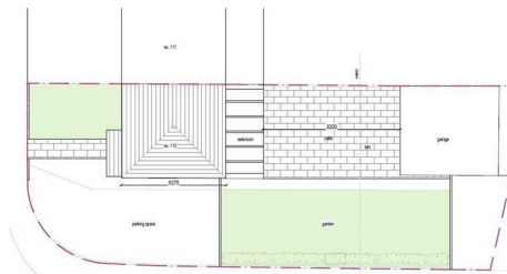
EXISTING SITE PLAN
